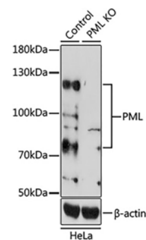
Fig. 2. Western blot analysis of extracts from normal (control) and PML knockout (KO) HeLa cells, using PML antibody at 1:1000 dilution. Secondary antibody: HRP-labeled Goat Anti-Rabbit IgG(H+L) (A0208) at 1:1000 dilution. Lysates/proteins: 25 \mu g per lane. Blocking buffer: QuickBlock TM Blocking Buffer (P0231). Detection: BeyoECL Star (P0018A). Exposure time:1s.
