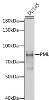
Fig. 1. Western blot analysis of extracts of various cell lines, using PML antibody at 1:1000 dilution. Secondary antibody: HRP-labeled Goat Anti-Rabbit IgG(H+L) (A0208) at 1:1000 dilution. Lysates/proteins: 25 \mu g per lane. Blocking buffer: QuickBlock TM Blocking Buffer (P0231).
