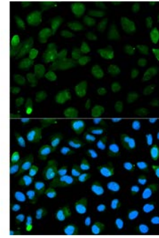
Fig. 4. Immunofluorescence analysis of HeLa cells using PML antibody. Blue: DAPI for nuclear staining.
