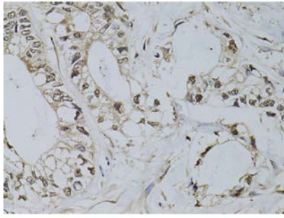
Fig. 3. Immunohistochemistry of paraffin-embedded human gastric cancer using PML antibody at dilution of 1:100 (40x lens).
